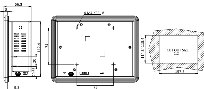
PPC-F06B-BT Dimensions (Unit: mm)
