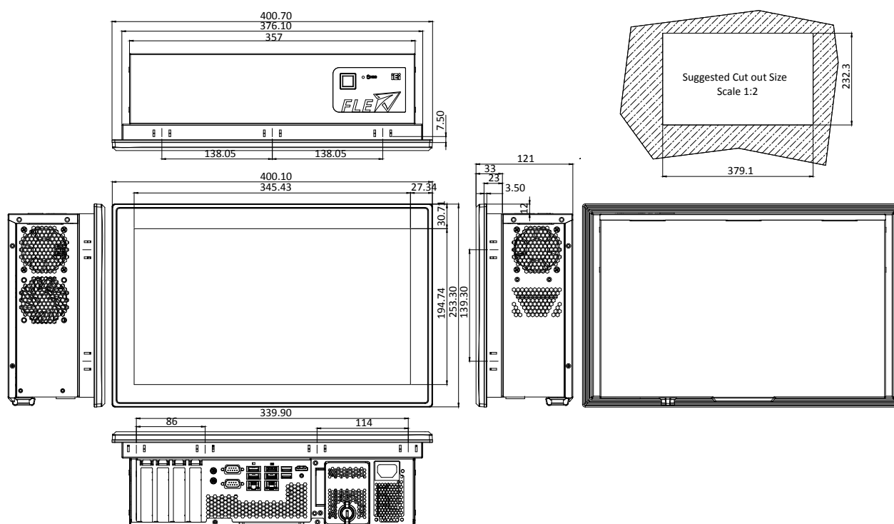
PPC-FW15C-Q370 Dimensions (Unit: mm)
