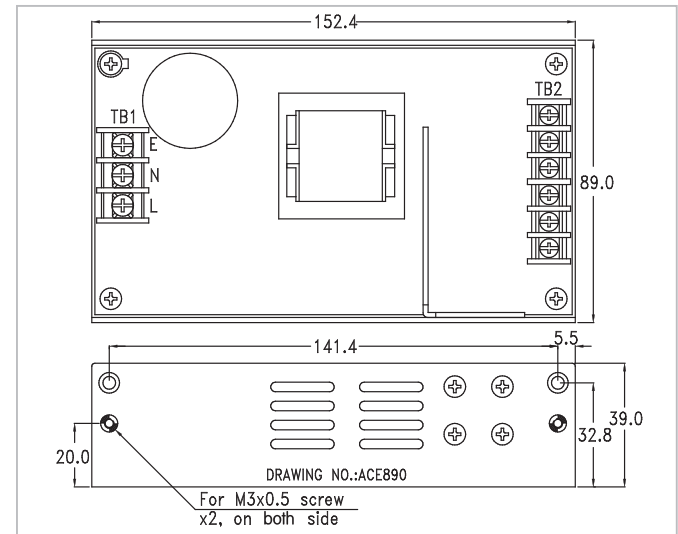
Dimensions (Unit: mm)
